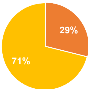
Proportion of market with 25% vesting at Threshold
